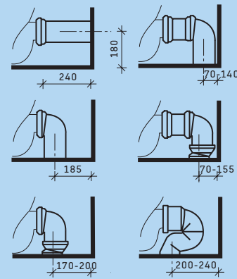
variants of Vario toilet
